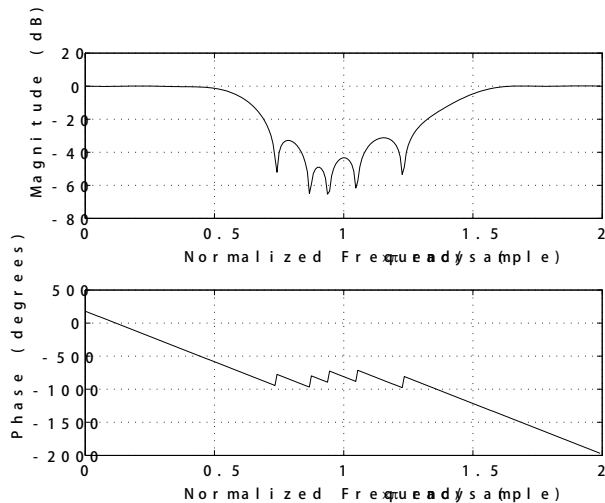
(a) Result of lowpass filter
